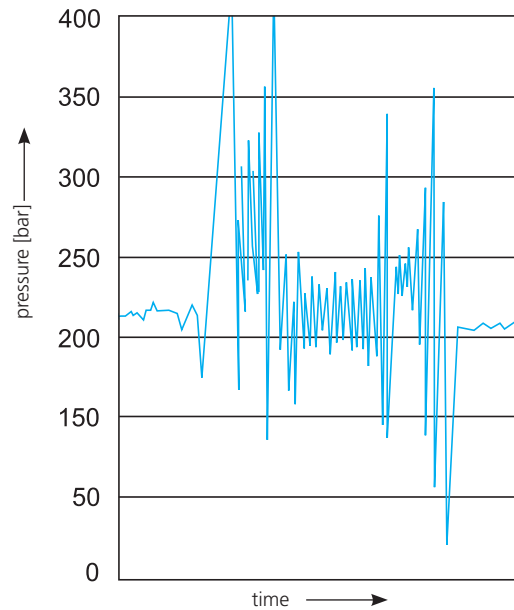
Pressure peaks
