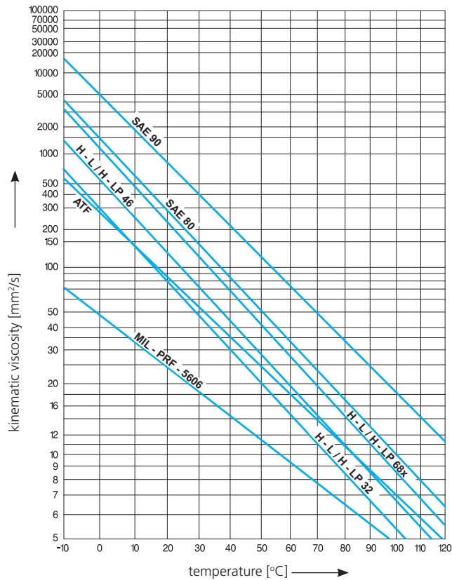
Viscosity
