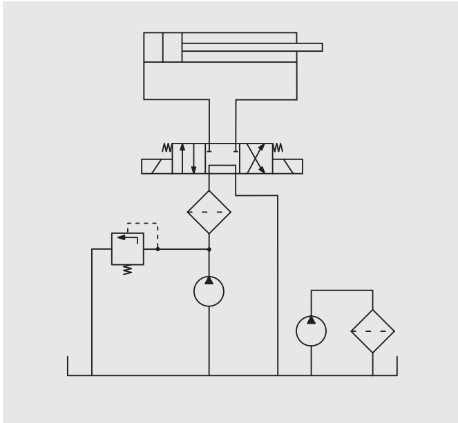
Hydraulic system with high-pressure filter and off-line filter unit
