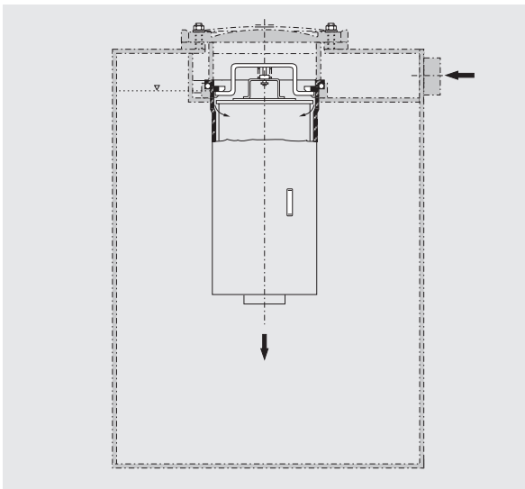
Return filter E 441 ... E 700 for installation in tanks
